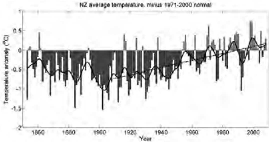
Figure 5. Adjusted average NZ temperatures from 1860 to 2000 as reported by NIWA. ( http://www.niwa.co.nz/our-science/climate/news/all/nz-temp-record )
